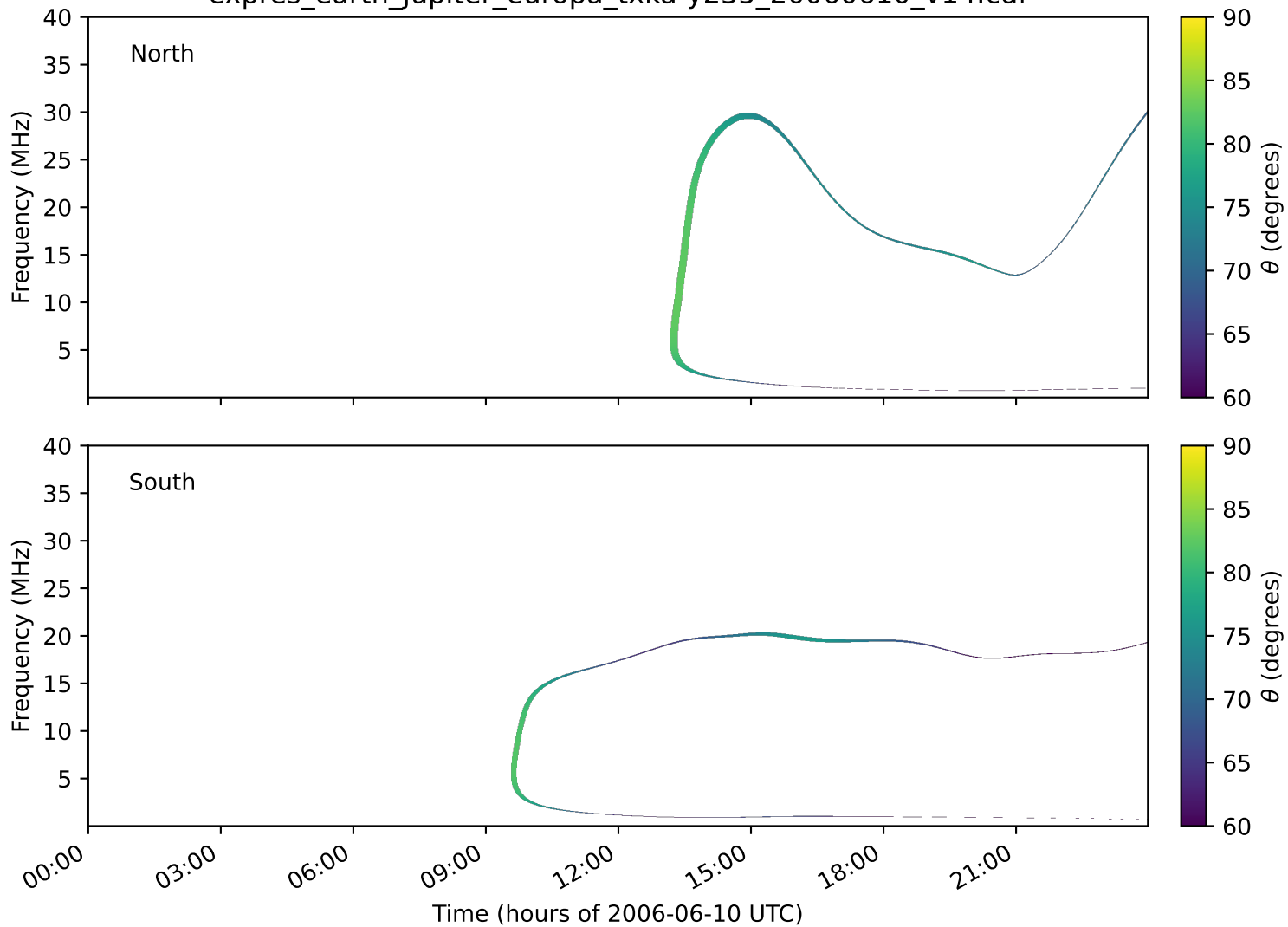
expres_earth_jupiter_europa_txka-y235_20060610_v14.cdf
