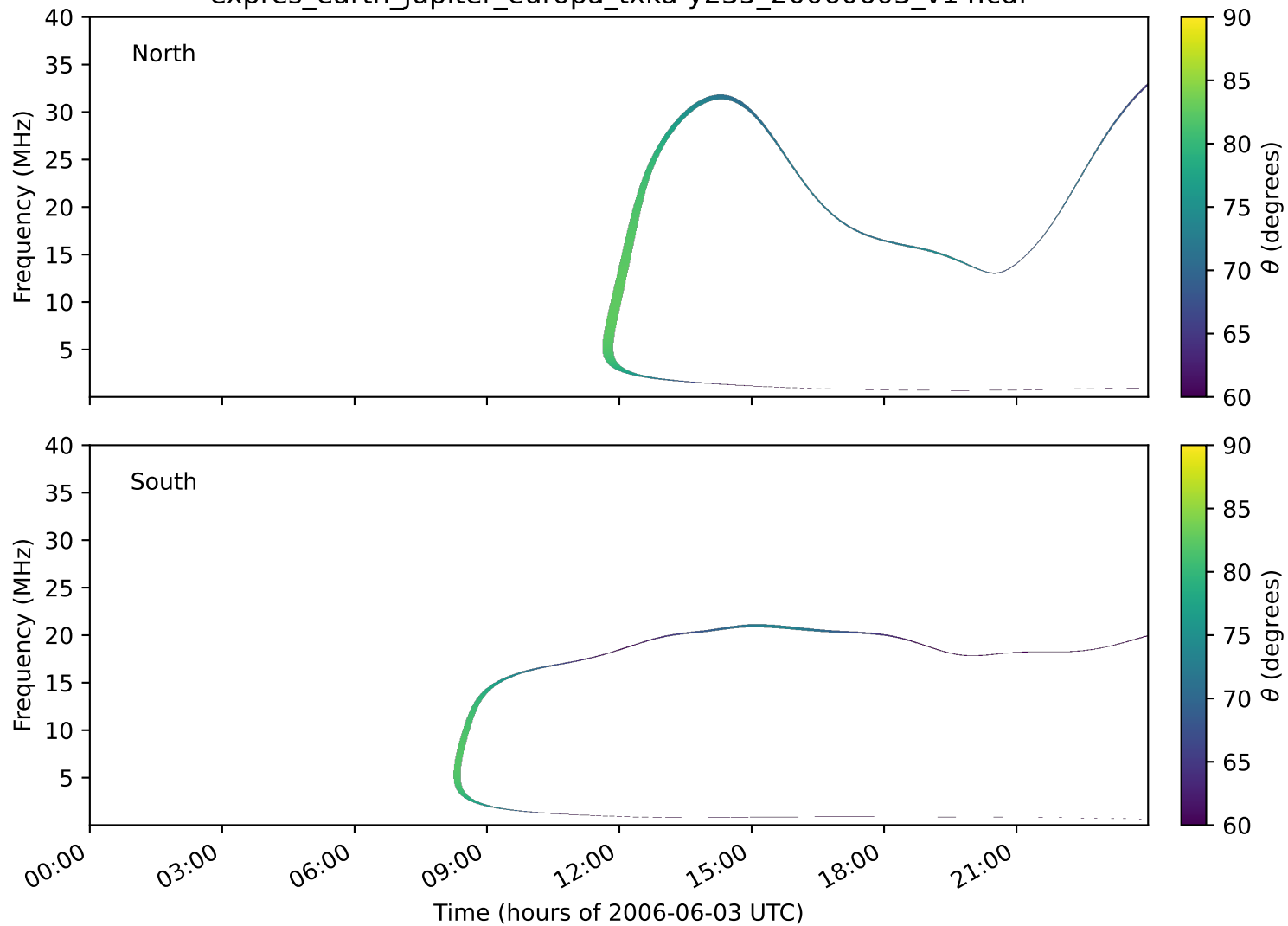
expres_earth_jupiter_europa_txka-y235_20060603_v14.cdf
