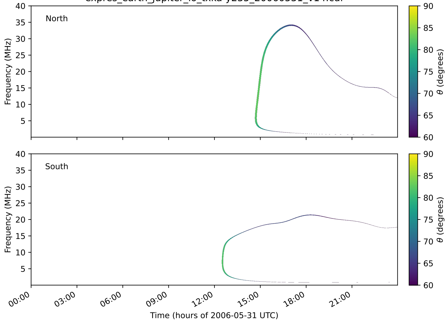
expres_earth_jupiter_io_txka-y235_20060531_v14.cdf
