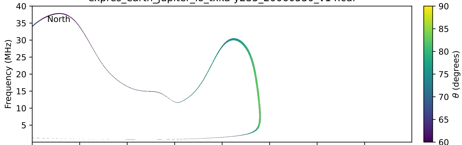
expres_earth_jupiter_io_txka-y235_20060530_v14.cdf
