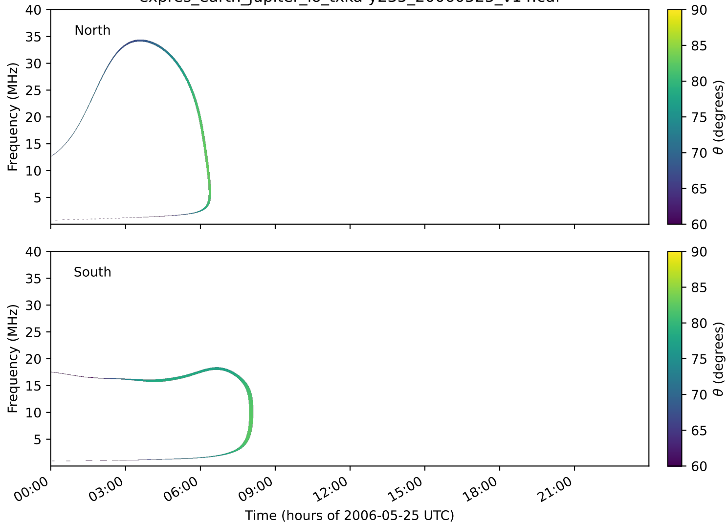
expres_earth_jupiter_io_txka-y235_20060525_v14.cdf
