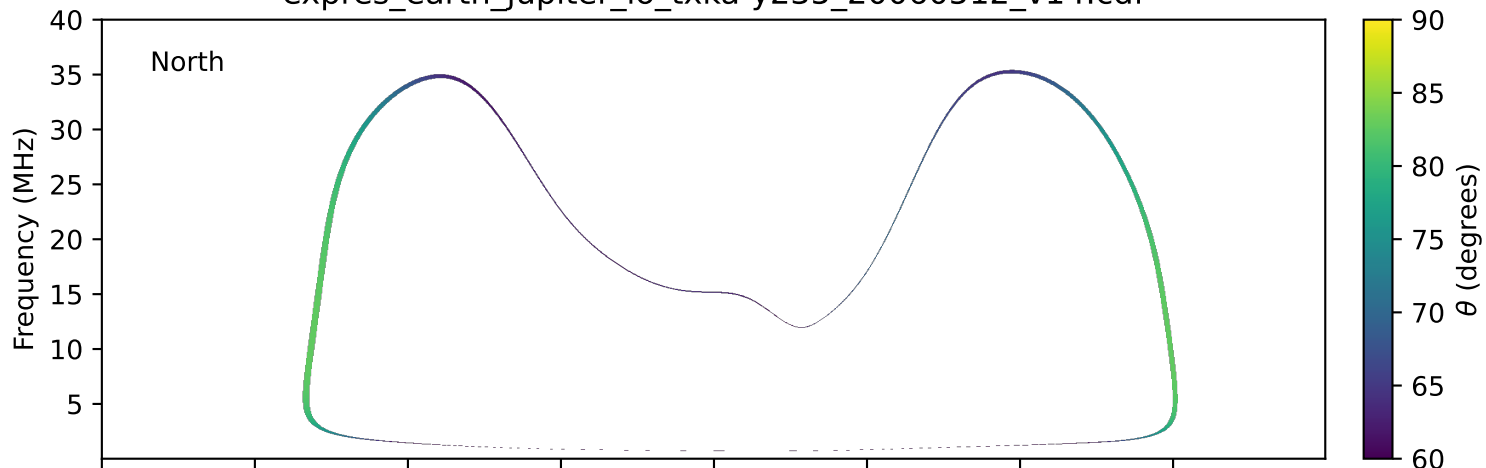
expres_earth_jupiter_io_txka-y235_20060512_v14.cdf
