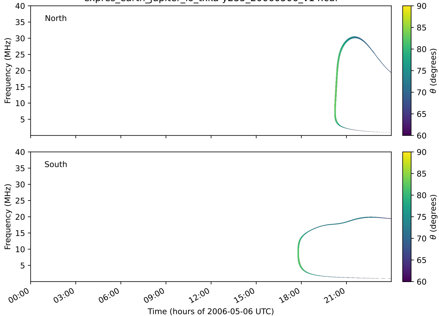
expres_earth_jupiter_io_txka-y235_20060506_v14.cdf
