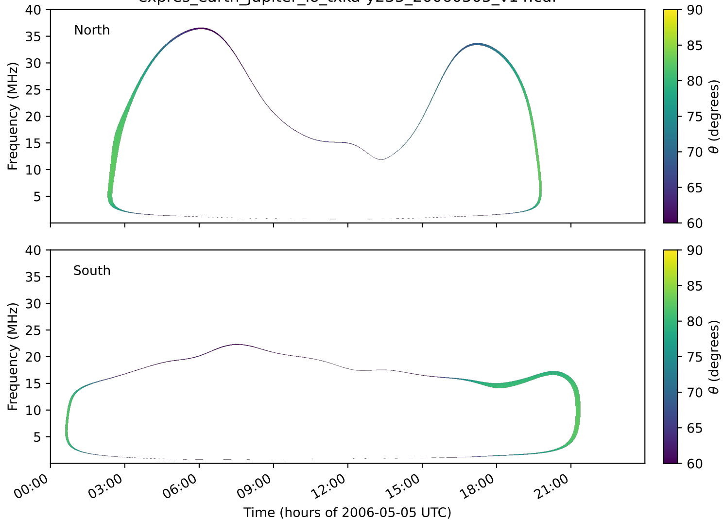
expres_earth_jupiter_io_txka-y235_20060505_v14.cdf
