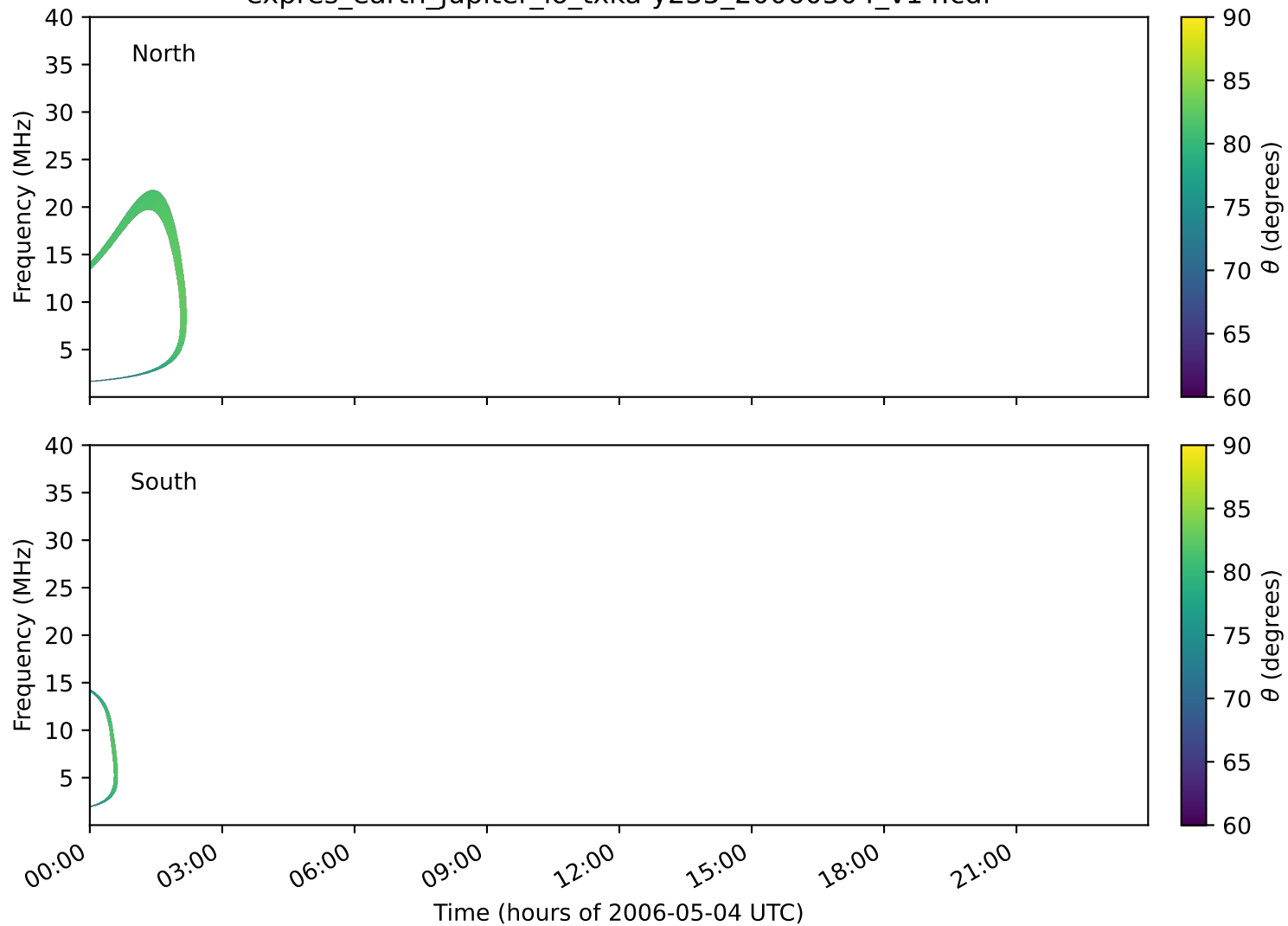
expres_earth_jupiter_io_txka-y235_20060504_v14.cdf
