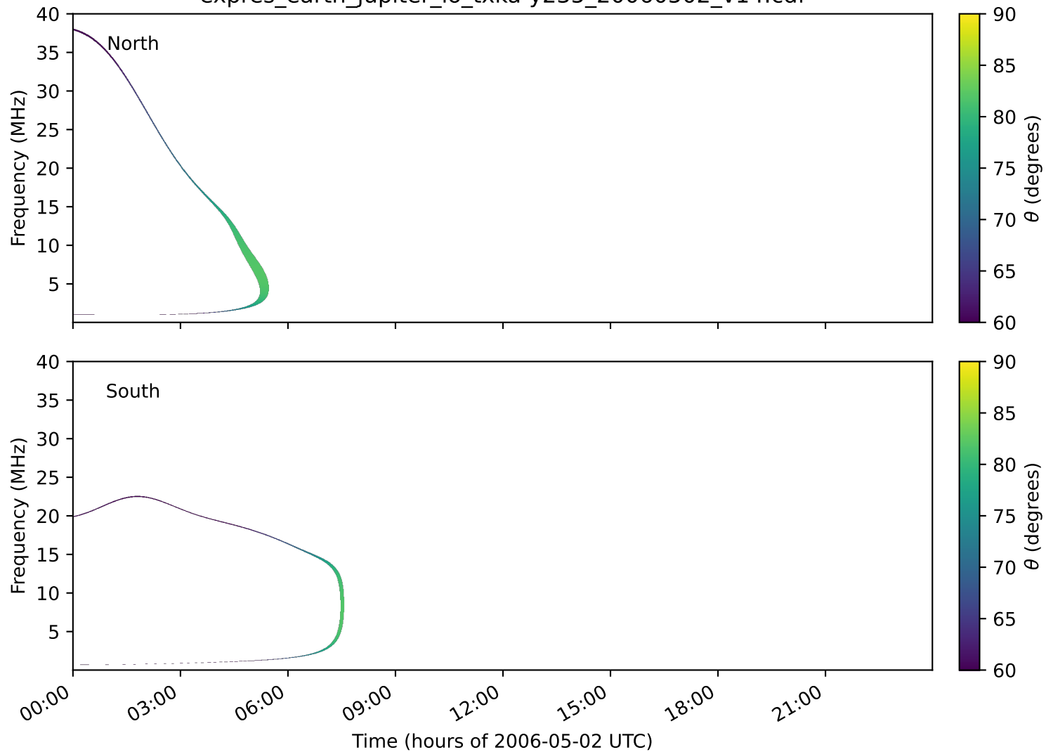
expres_earth_jupiter_io_txka-y235_20060502_v14.cdf
