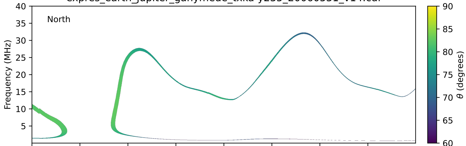
expres_earth_jupiter_ganymede_txka-y235_20060531_v14.cdf
