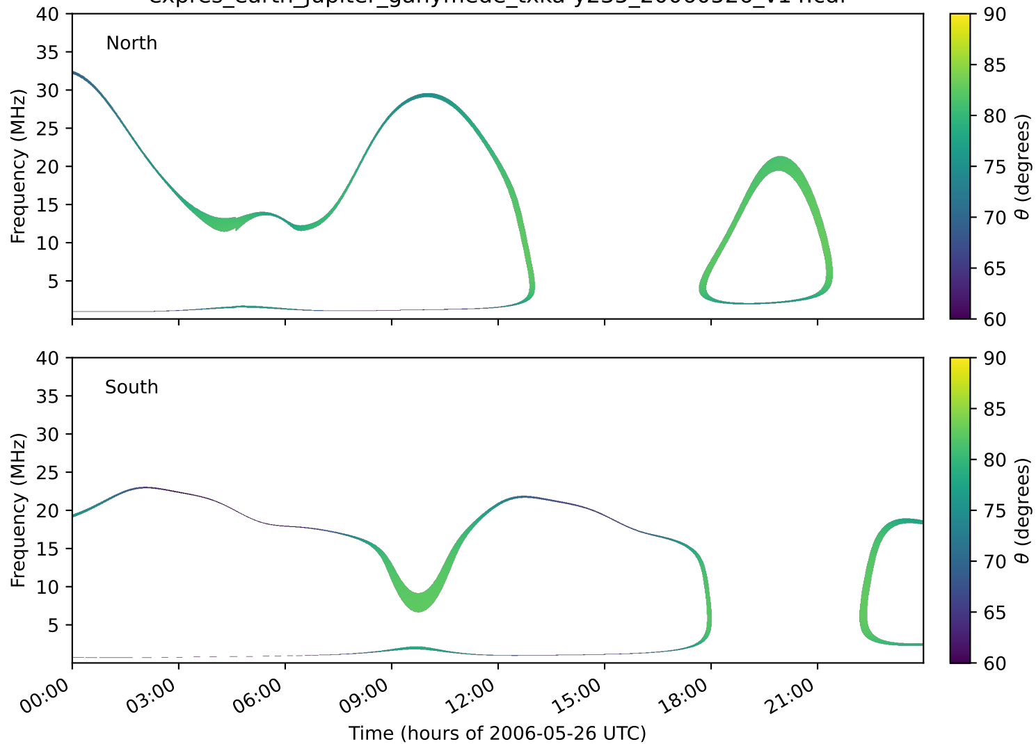
expres_earth_jupiter_ganymede_txka-y235_20060526_v14.cdf
