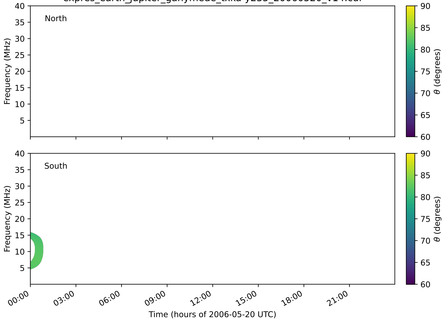
expres_earth_jupiter_ganymede_txka-y235_20060520_v14.cdf
