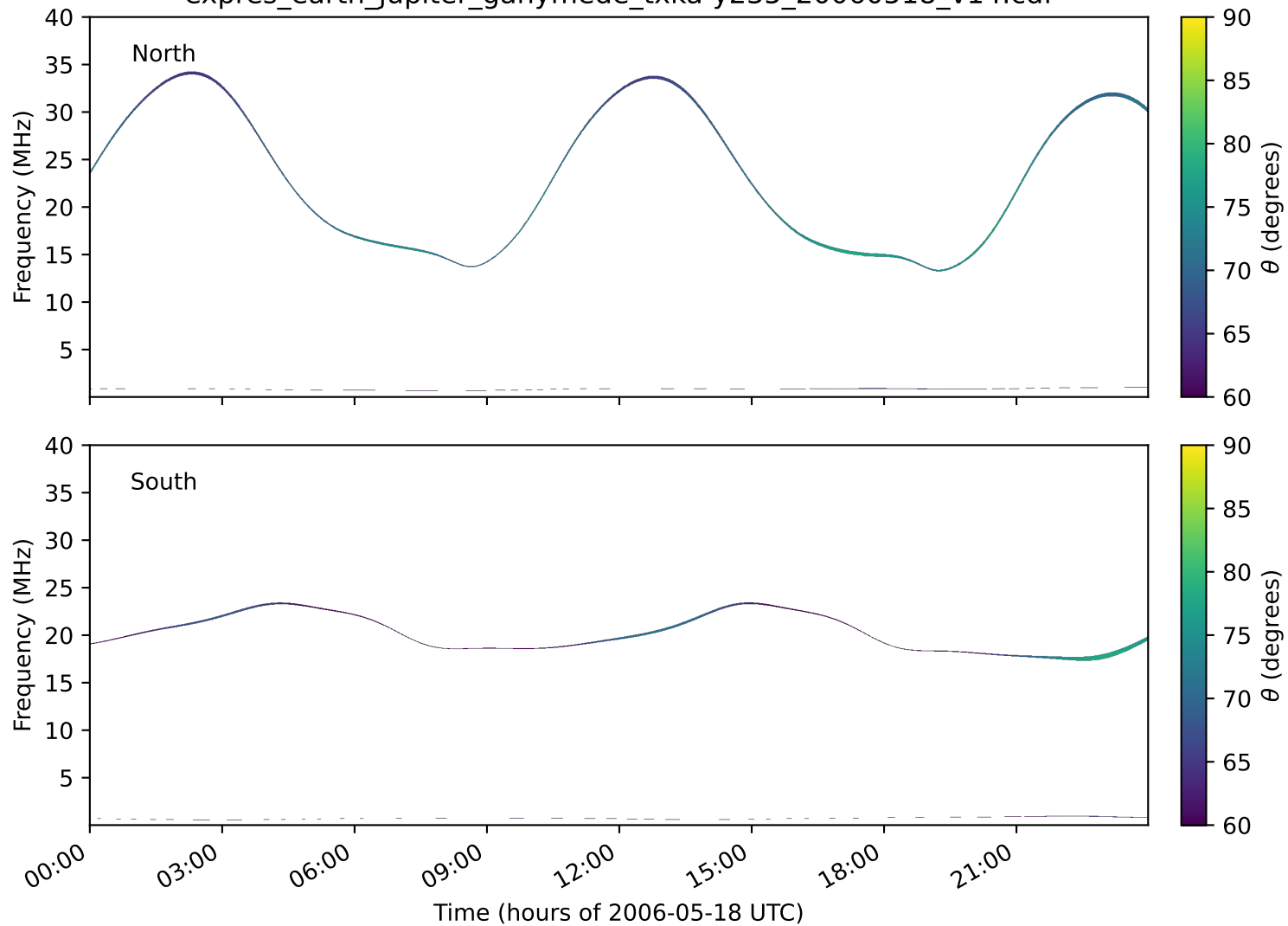
expres_earth_jupiter_ganymede_txka-y235_20060518_v14.cdf
