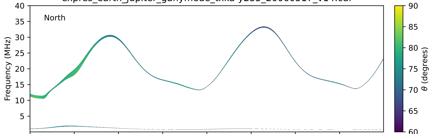
expres_earth_jupiter_ganymede_txka-y235_20060517_v14.cdf
