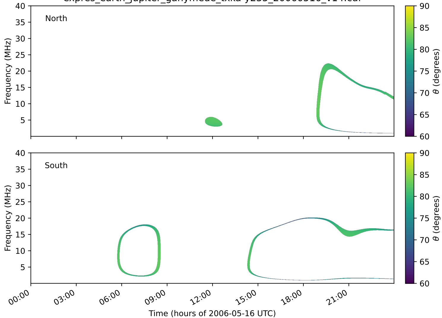
expres_earth_jupiter_ganymede_txka-y235_20060516_v14.cdf
