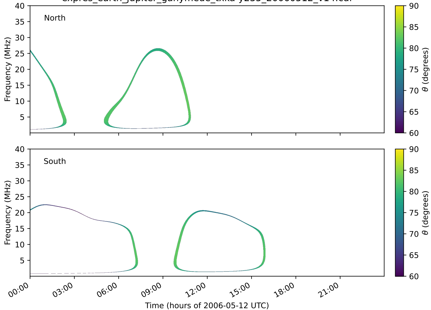
expres_earth_jupiter_ganymede_txka-y235_20060512_v14.cdf
