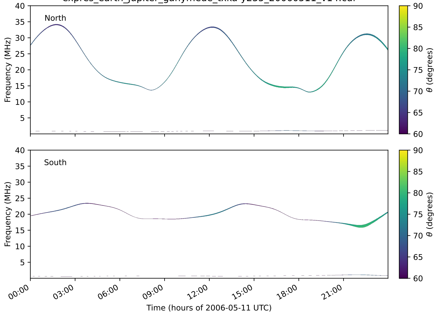
expres_earth_jupiter_ganymede_txka-y235_20060511_v14.cdf
