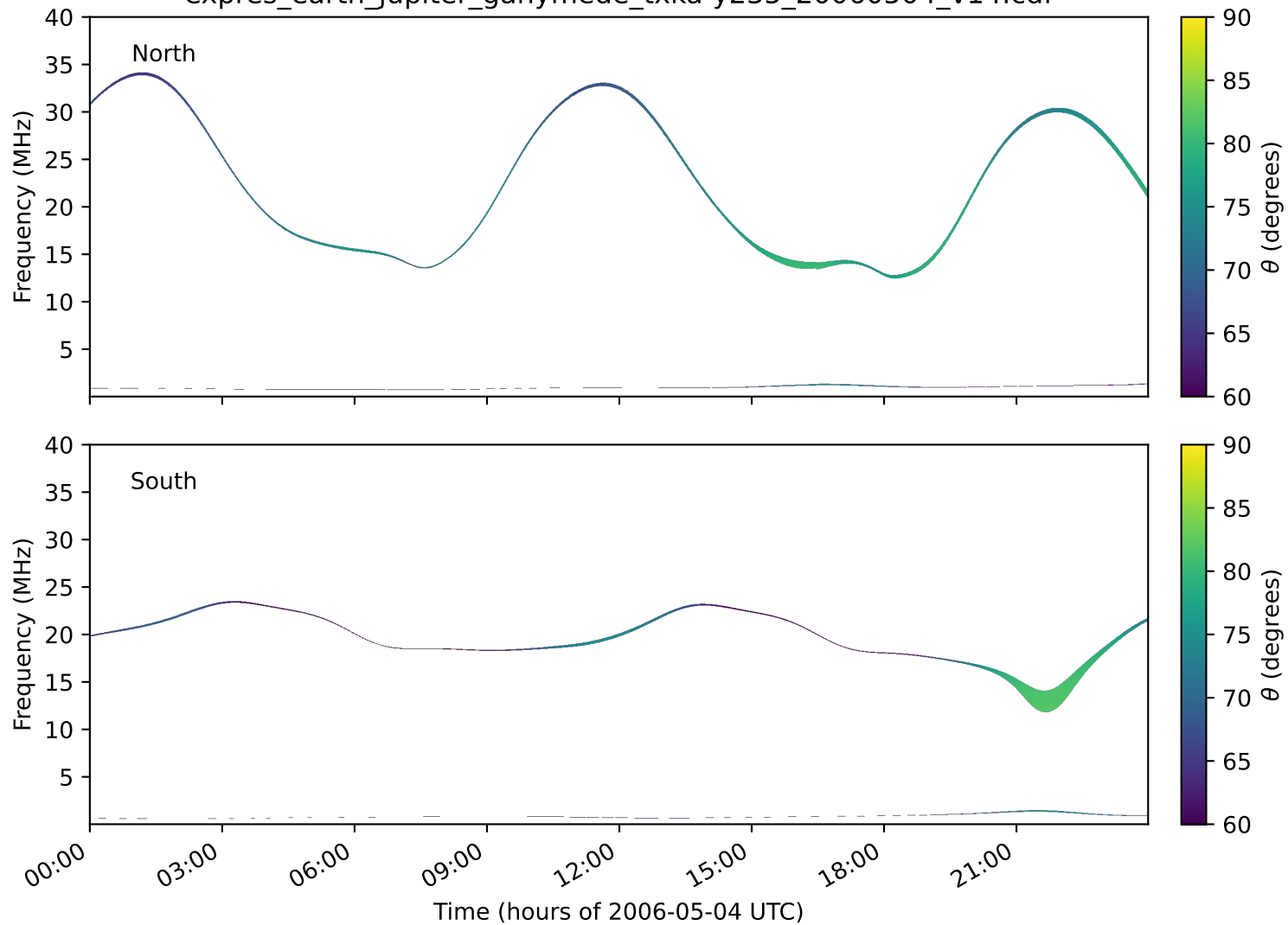
expres_earth_jupiter_ganymede_txka-y235_20060504_v14.cdf
