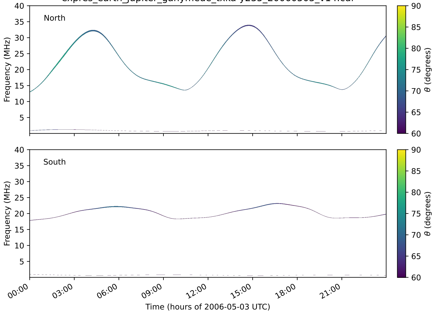
expres_earth_jupiter_ganymede_txka-y235_20060503_v14.cdf
