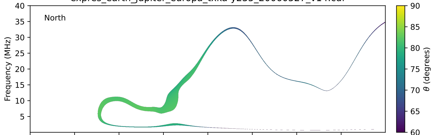
expres_earth_jupiter_europa_txka-y235_20060527_v14.cdf
