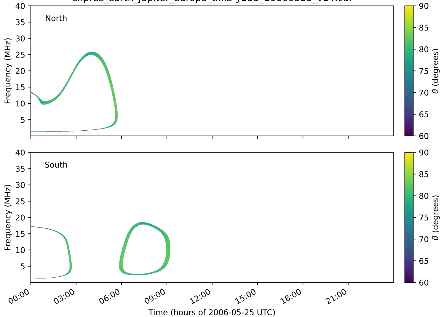
expres_earth_jupiter_europa_txka-y235_20060525_v14.cdf
