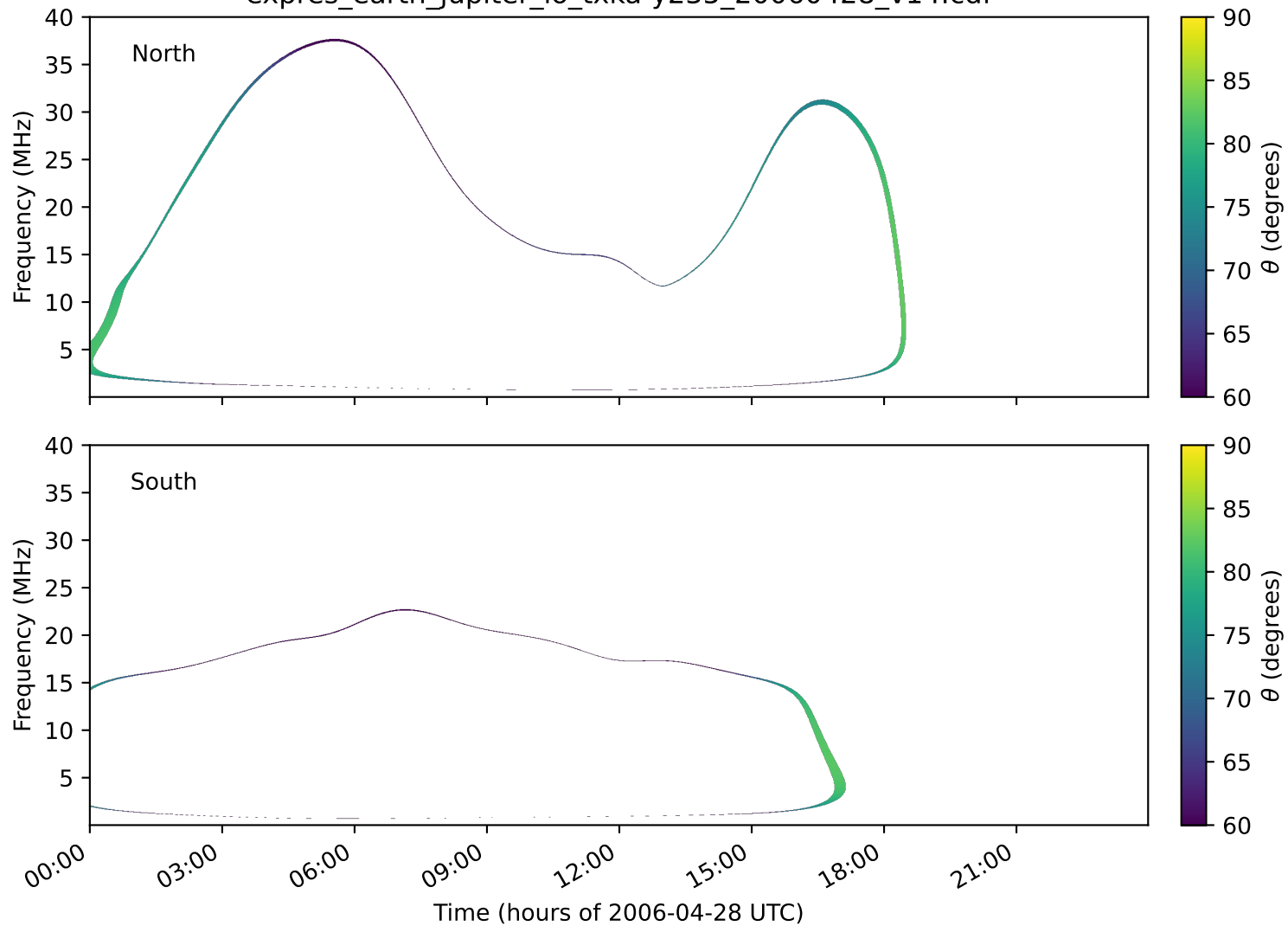
expres_earth_jupiter_io_txka-y235_20060428_v14.cdf
