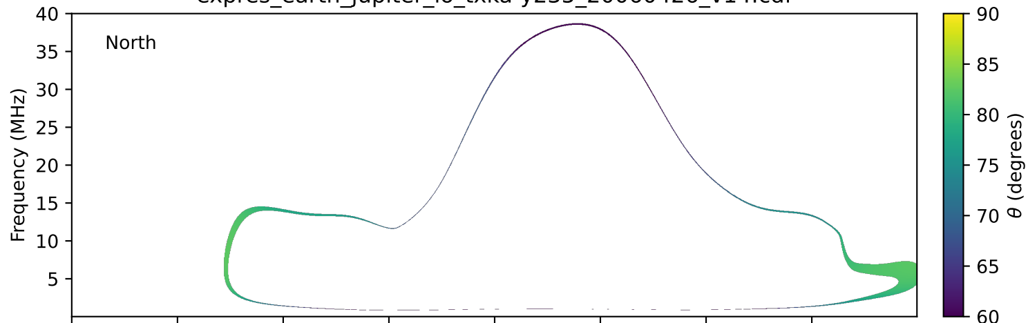
expres_earth_jupiter_io_txka-y235_20060426_v14.cdf
