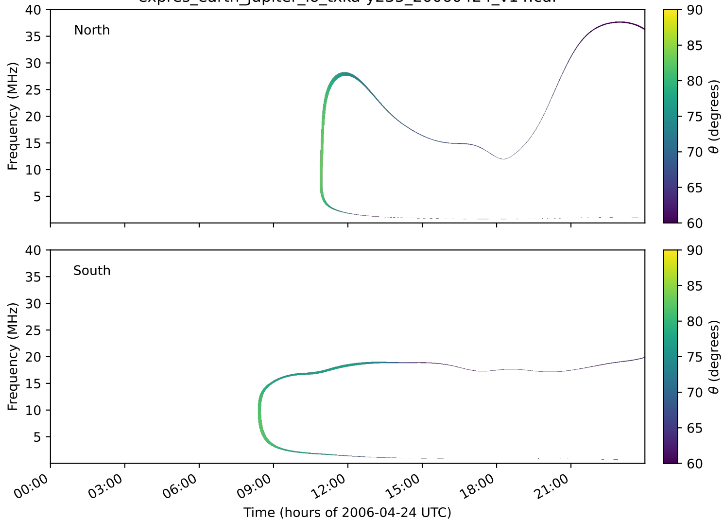
expres_earth_jupiter_io_txka-y235_20060424_v14.cdf
