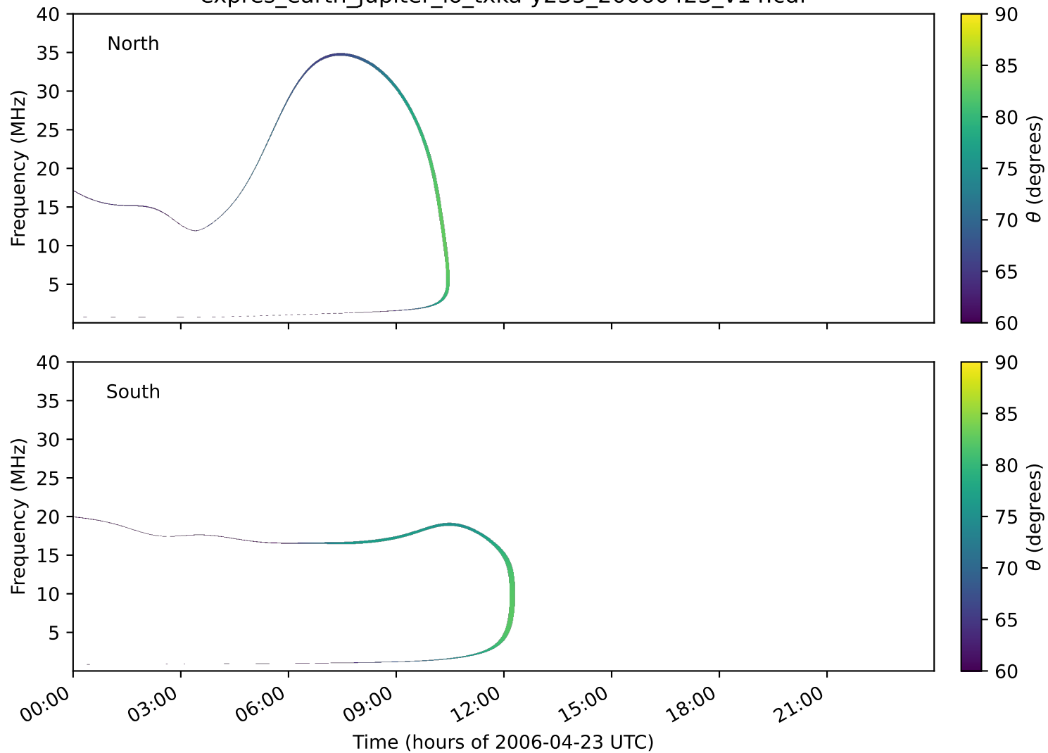
expres_earth_jupiter_io_txka-y235_20060423_v14.cdf
