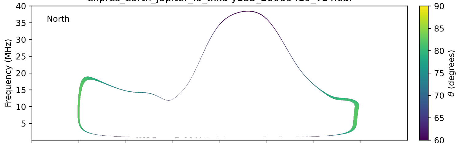
expres_earth_jupiter_io_txka-y235_20060419_v14.cdf
