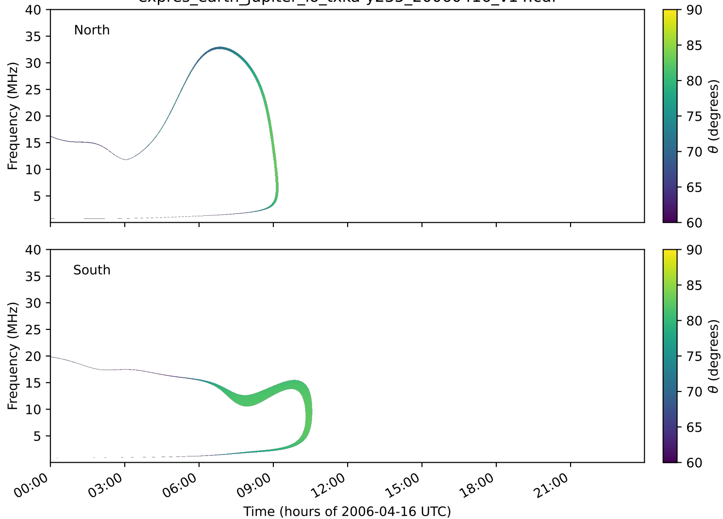
expres_earth_jupiter_io_txka-y235_20060416_v14.cdf
