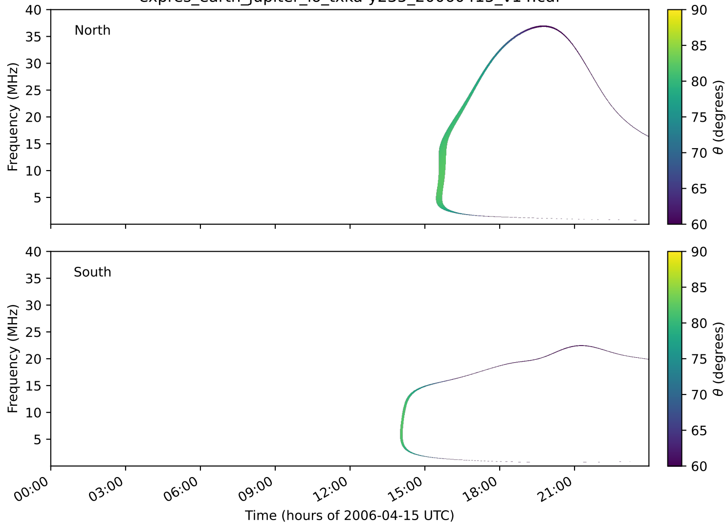
expres_earth_jupiter_io_txka-y235_20060415_v14.cdf
