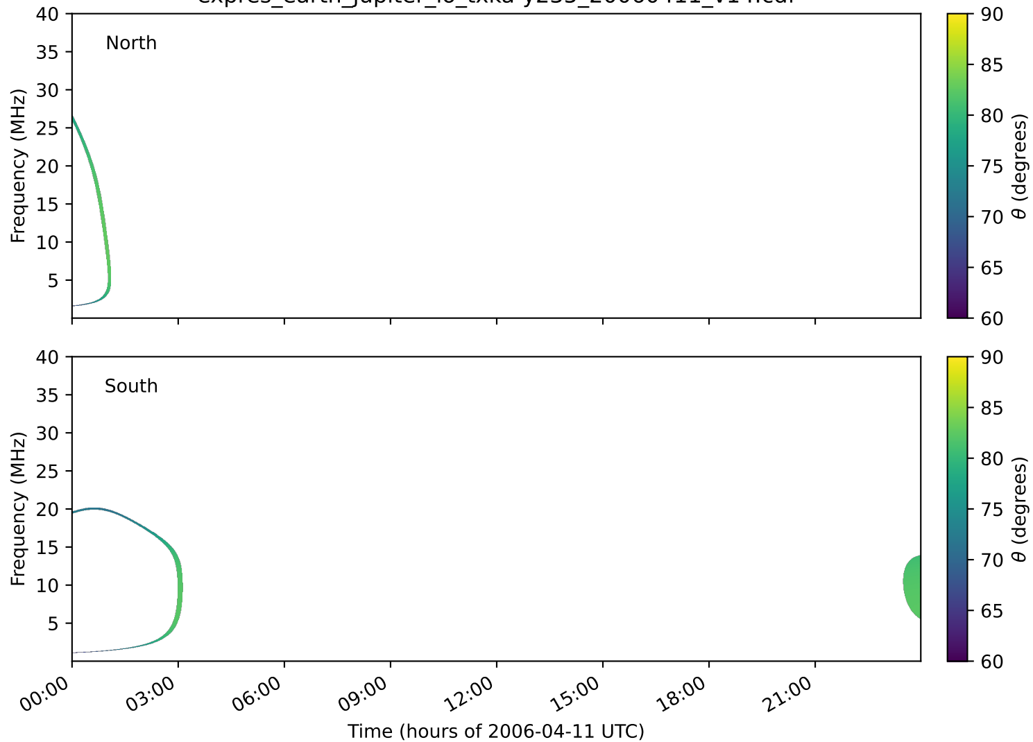
expres_earth_jupiter_io_txka-y235_20060411_v14.cdf
