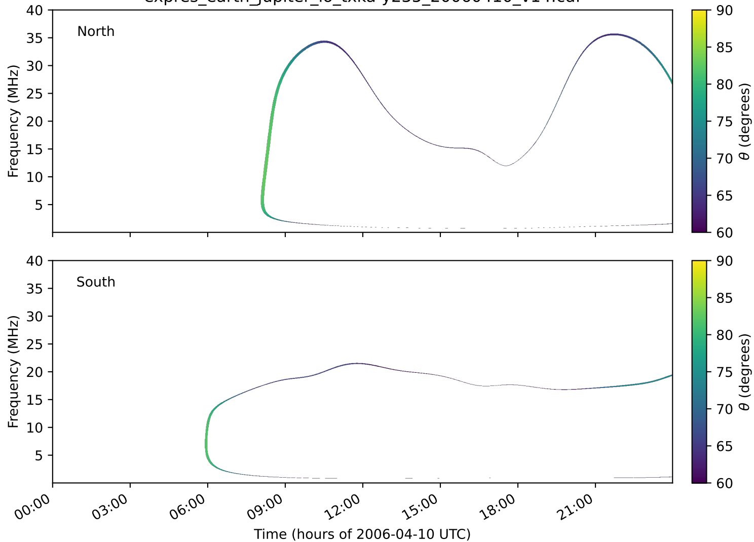
expres_earth_jupiter_io_txka-y235_20060410_v14.cdf
