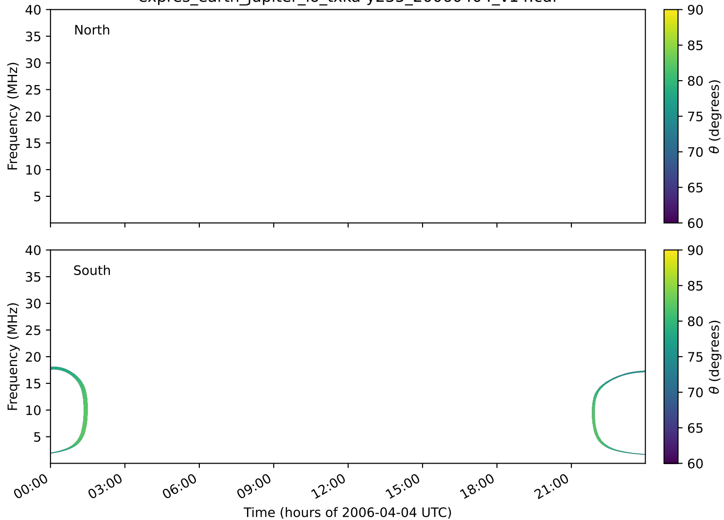
expres_earth_jupiter_io_txka-y235_20060404_v14.cdf
