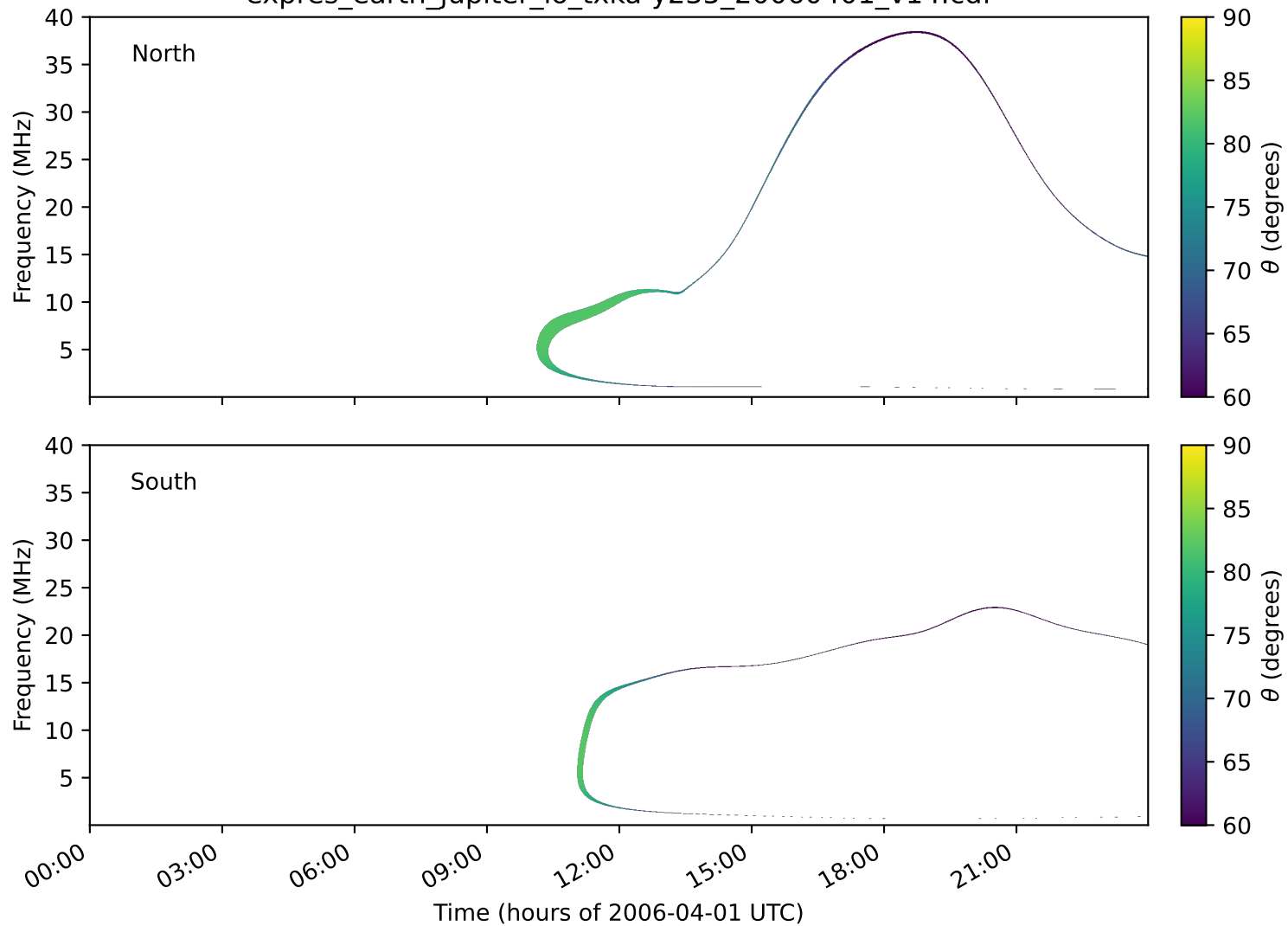
expres_earth_jupiter_io_txka-y235_20060401_v14.cdf
