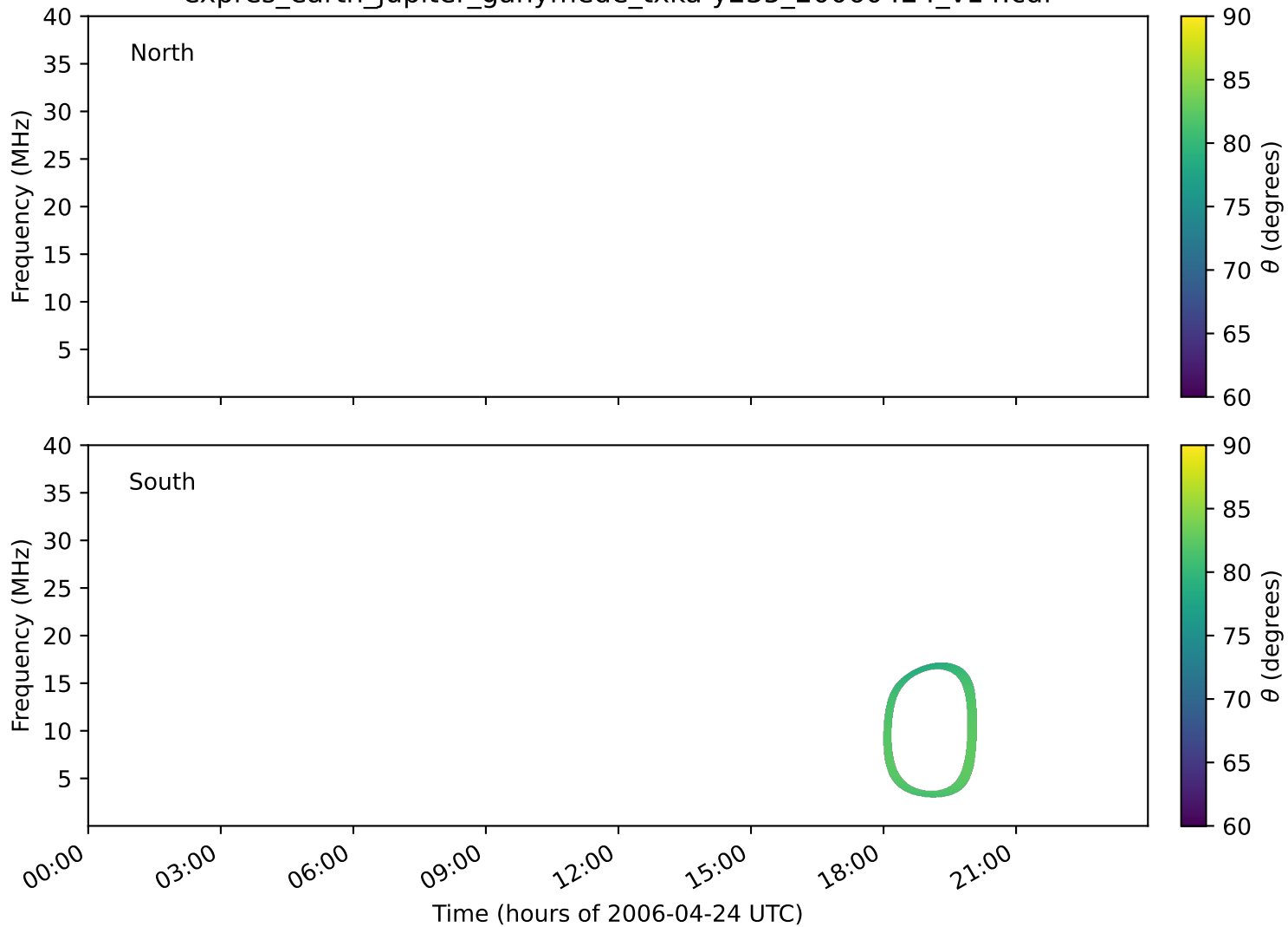
expres_earth_jupiter_ganymede_txka-y235_20060424_v14.cdf
