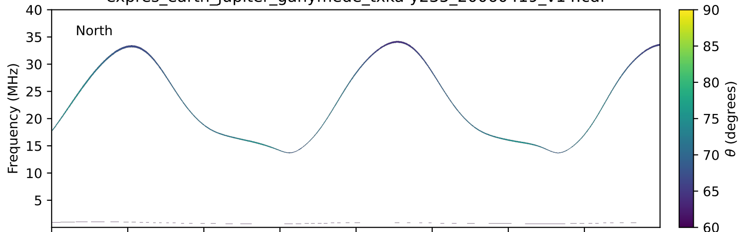
expres_earth_jupiter_ganymede_txka-y235_20060419_v14.cdf
