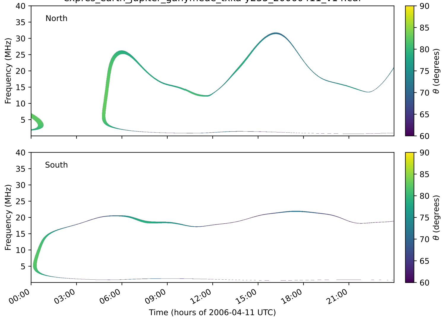
expres_earth_jupiter_ganymede_txka-y235_20060411_v14.cdf
