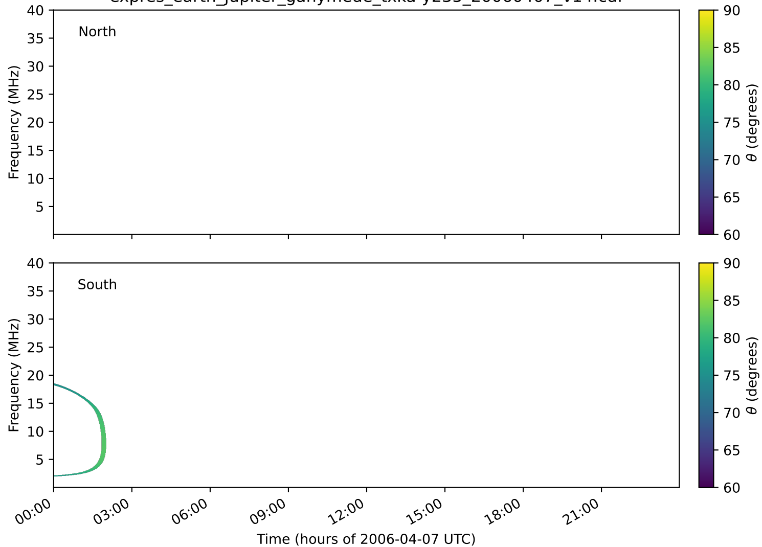
expres_earth_jupiter_ganymede_txka-y235_20060407_v14.cdf
