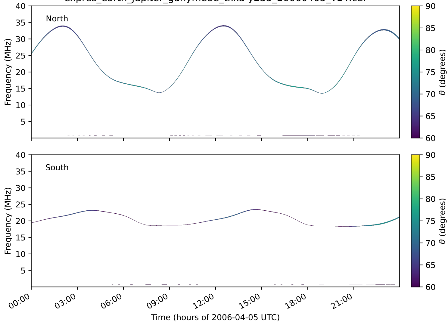
expres_earth_jupiter_ganymede_txka-y235_20060405_v14.cdf
