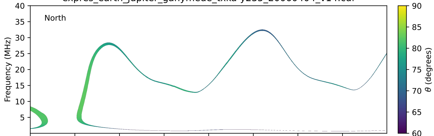
expres_earth_jupiter_ganymede_txka-y235_20060404_v14.cdf
