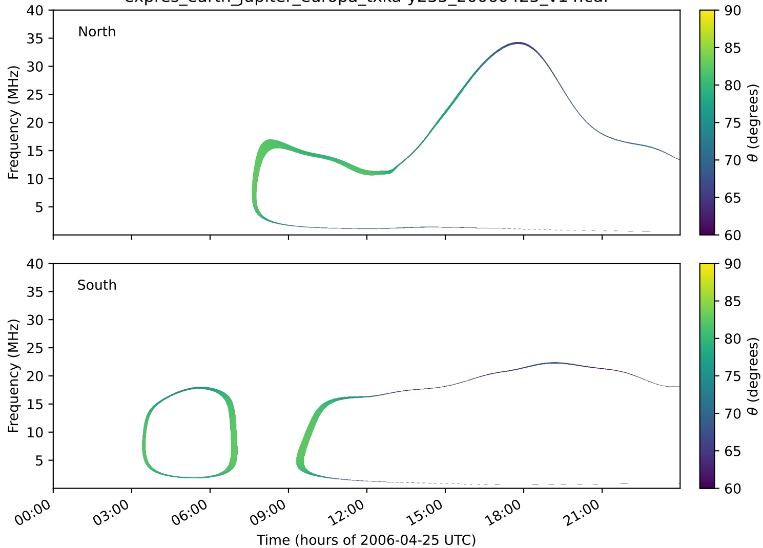
expres_earth_jupiter_europa_txka-y235_20060425_v14.cdf
