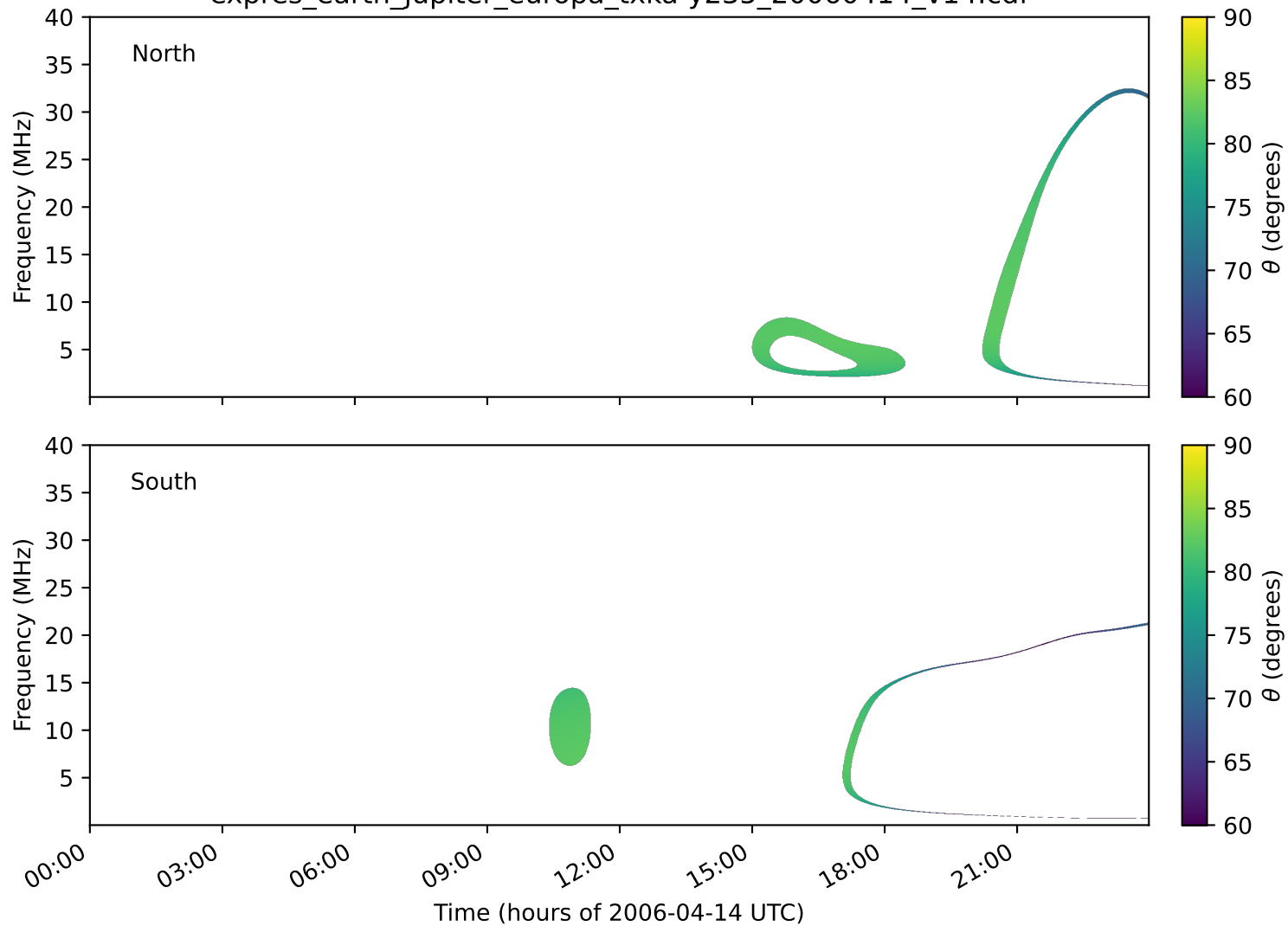
expres_earth_jupiter_europa_txka-y235_20060414_v14.cdf
