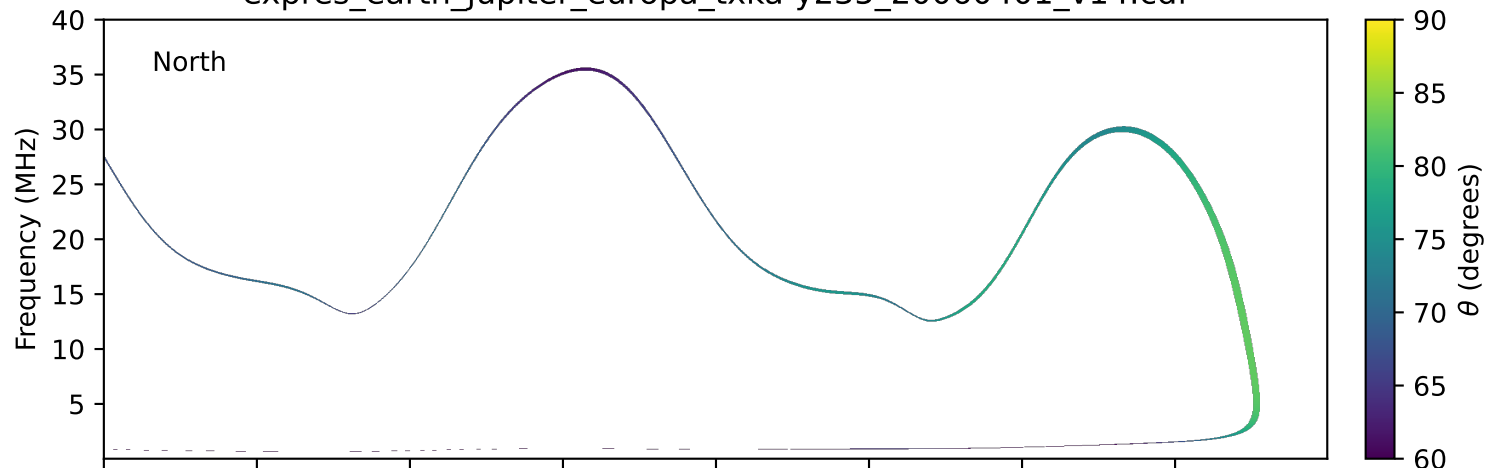
expres_earth_jupiter_europa_txka-y235_20060401_v14.cdf
