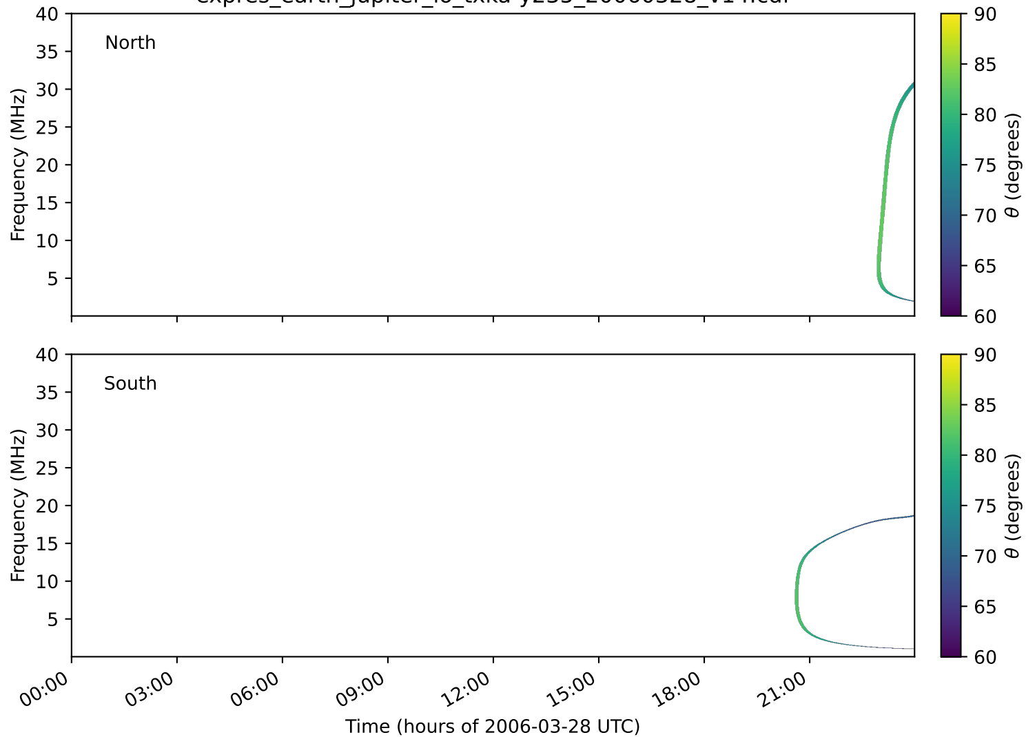
expres_earth_jupiter_io_txka-y235_20060328_v14.cdf
