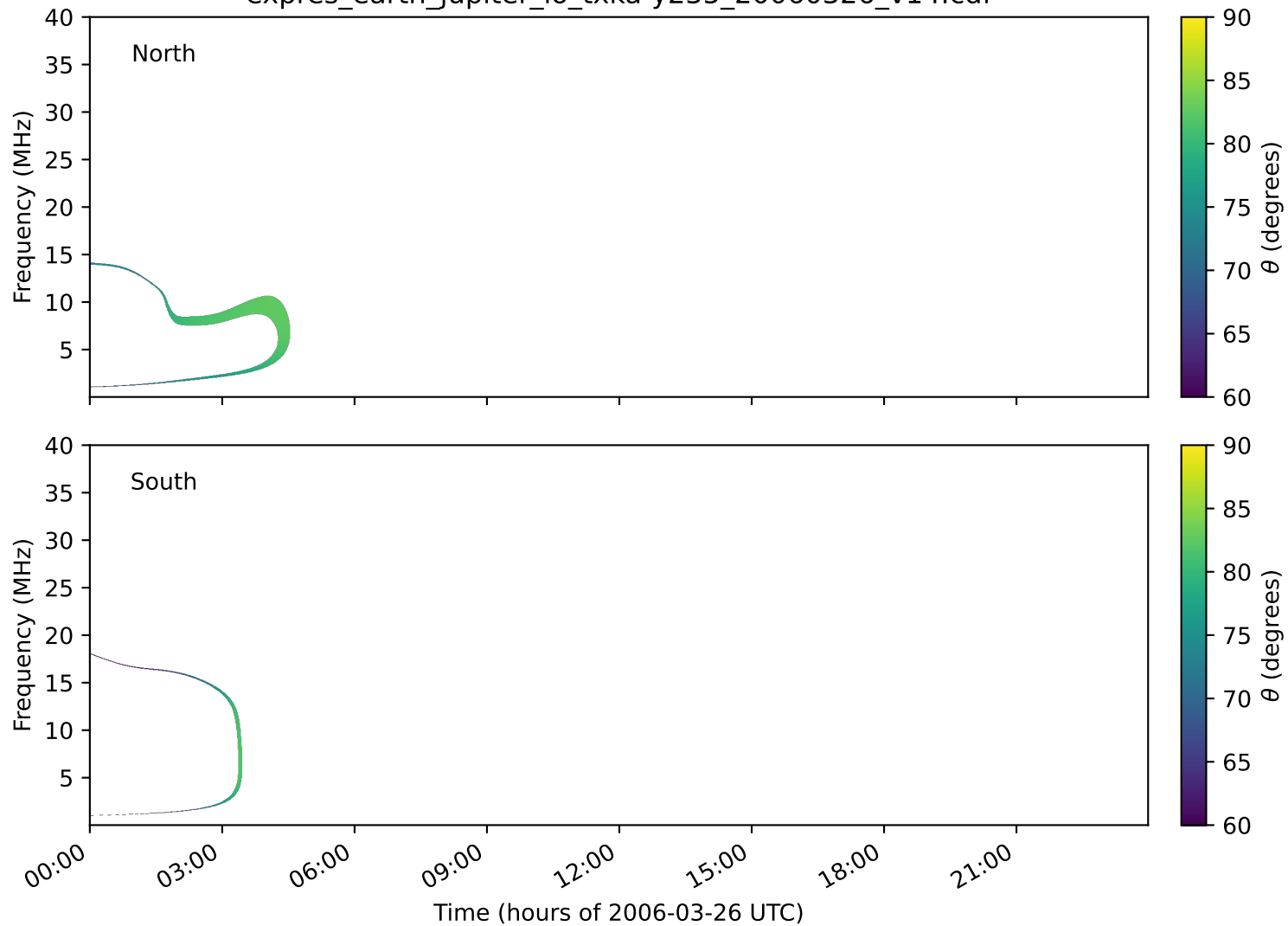
expres_earth_jupiter_io_txka-y235_20060326_v14.cdf
