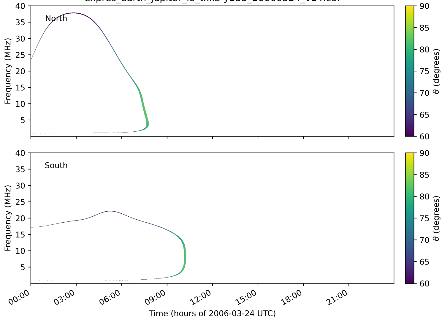
expres_earth_jupiter_io_txka-y235_20060324_v14.cdf
