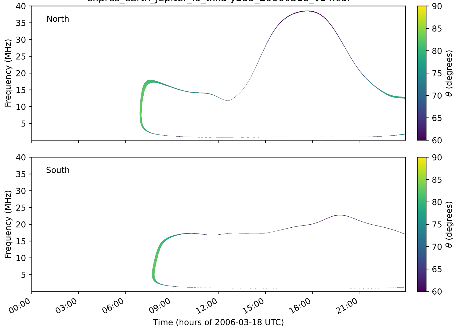
expres_earth_jupiter_io_txka-y235_20060318_v14.cdf
