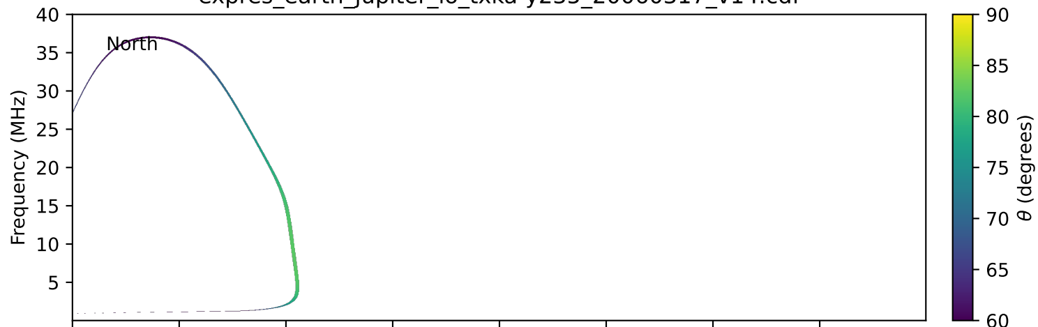
expres_earth_jupiter_io_txka-y235_20060317_v14.cdf
