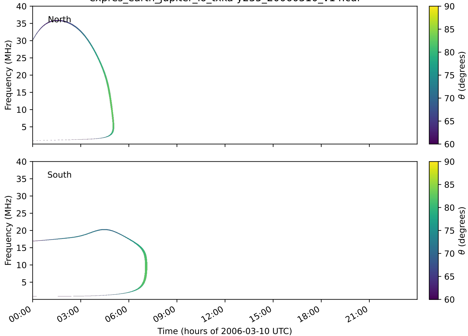
expres_earth_jupiter_io_txka-y235_20060310_v14.cdf
