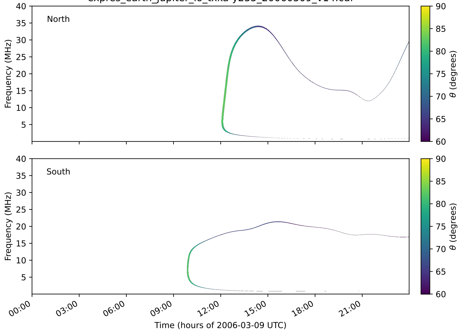
expres_earth_jupiter_io_txka-y235_20060309_v14.cdf
