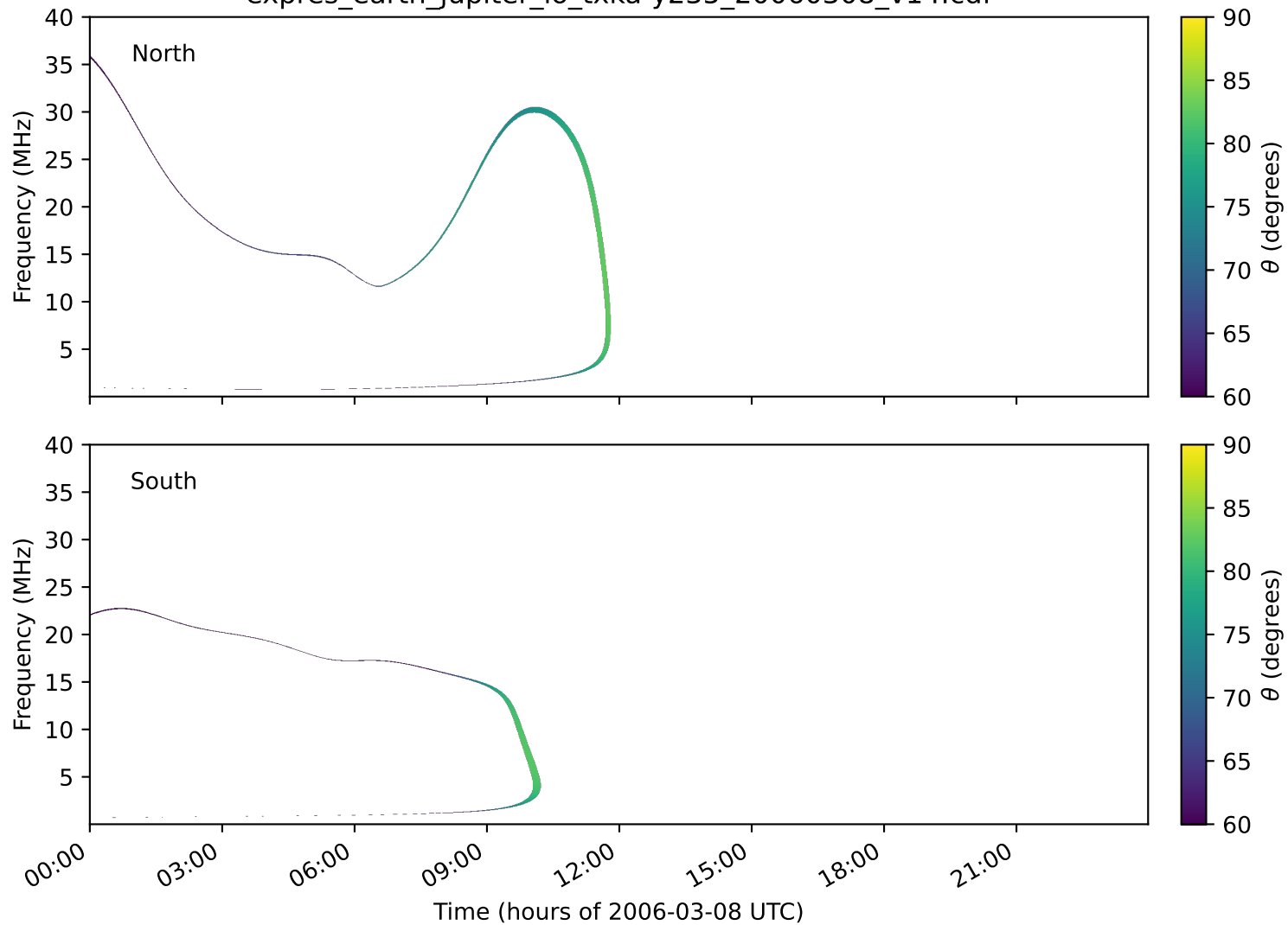
expres_earth_jupiter_io_txka-y235_20060308_v14.cdf
